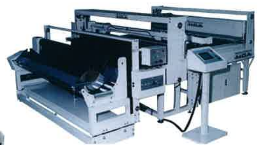
バケット式強制解反装置 (自動耳揃え装置付き) Bucket type Forcing Unwinding Device ( Installed Auto, Fabric Edge Control Device )
